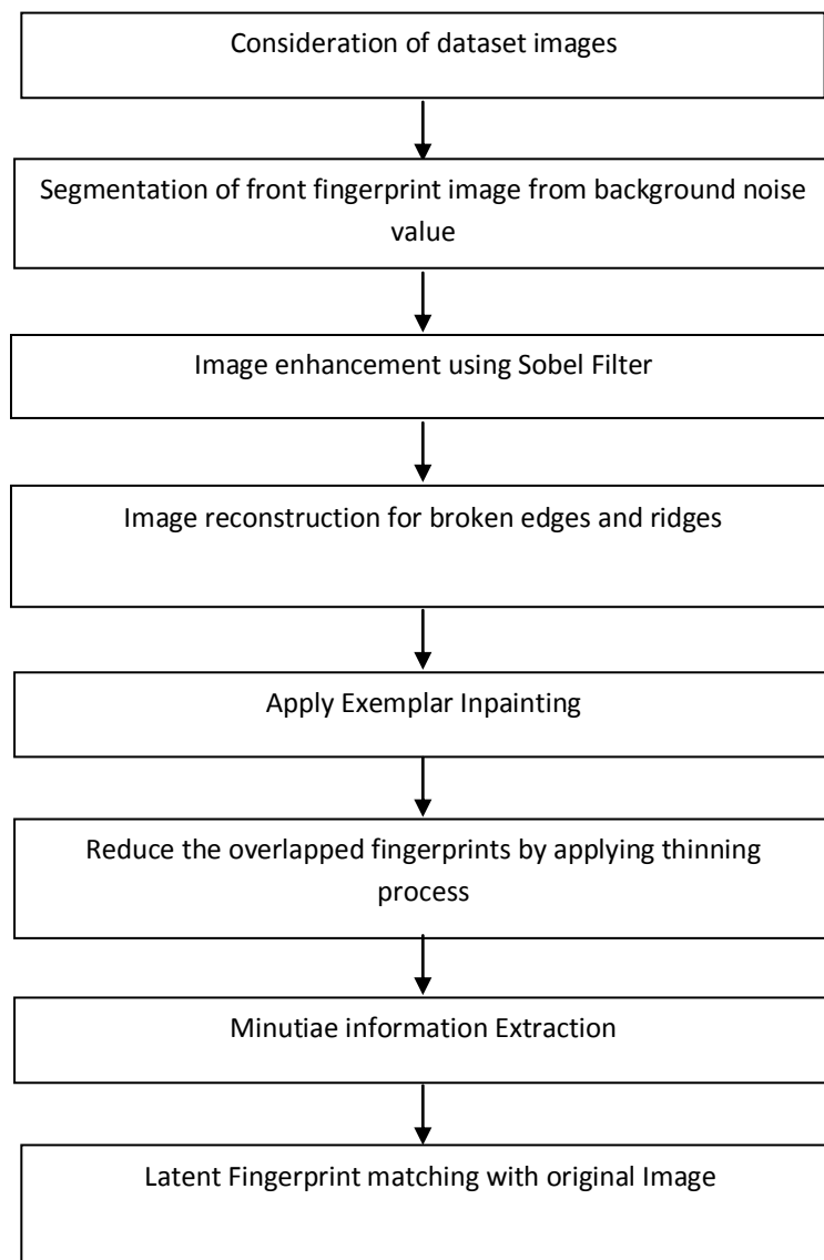
Figure 2: Latent fingerprint Enhancement, Reconstruction and Recognition using Exemplar Inpainting
